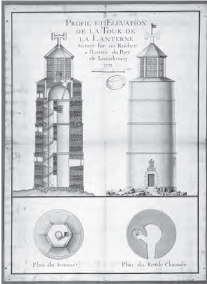
◀ FR CAOM COL C 11 B 39 Plan for the Louisbourg Lighthouse, 1733 Plan du phare de Louisbourg 1733
